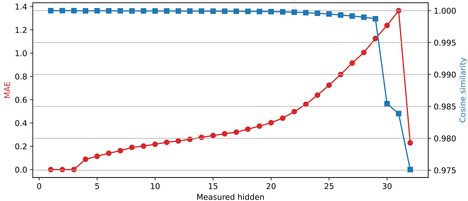
Phi-3-mini-4k-instruct | Quantized layer 3 | float64 → int2
