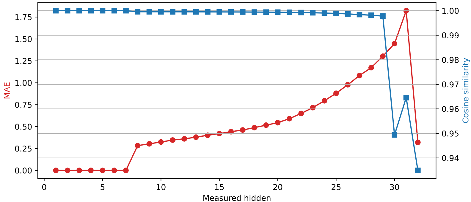
Phi-3-mini-4k-instruct | Quantized layer 7 | float64 → int2
