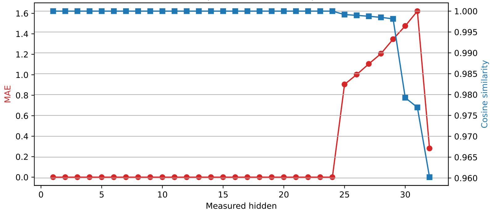
Phi-3-mini-4k-instruct | Quantized layer 24 | float64 → int2
