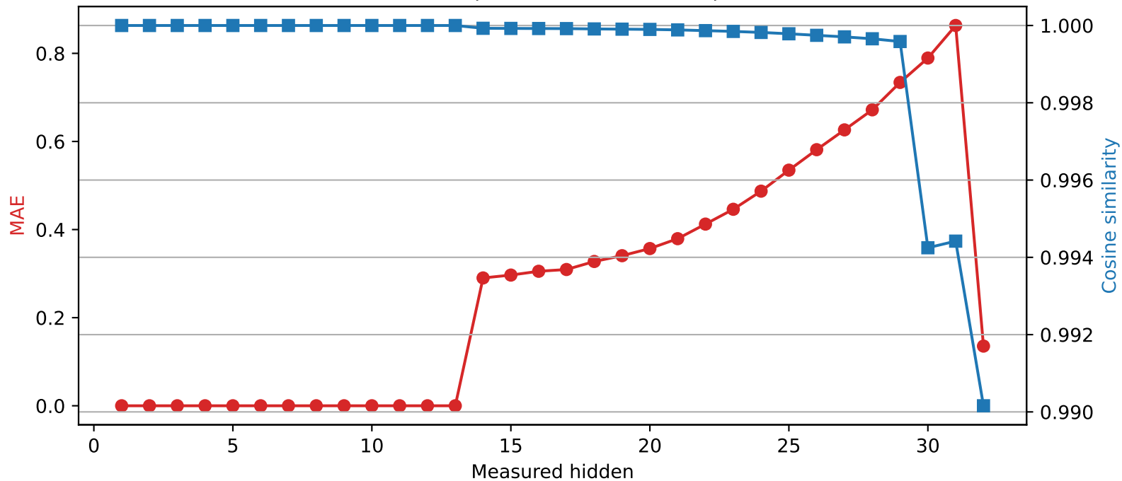
Phi-3-mini-4k-instruct | Quantized layer 13 | float64 \rightarrow int2
