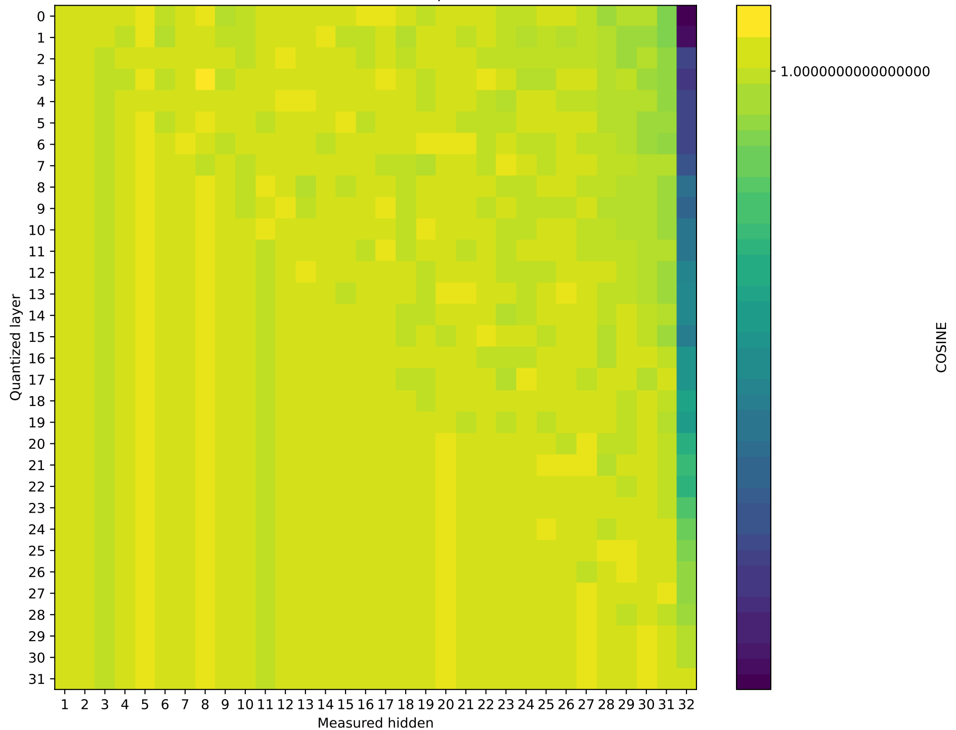
Model: Mistral-7B-Instruct-v0.3 | float64 → int32
