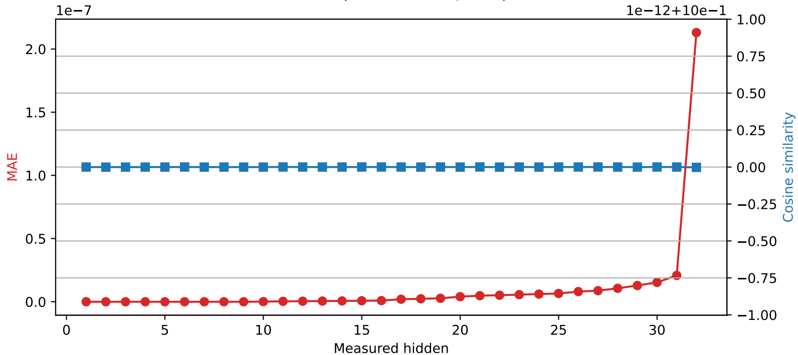
Mistral-7B-Instruct-v0.3 | Quantized layer 9 | float64 → int32
