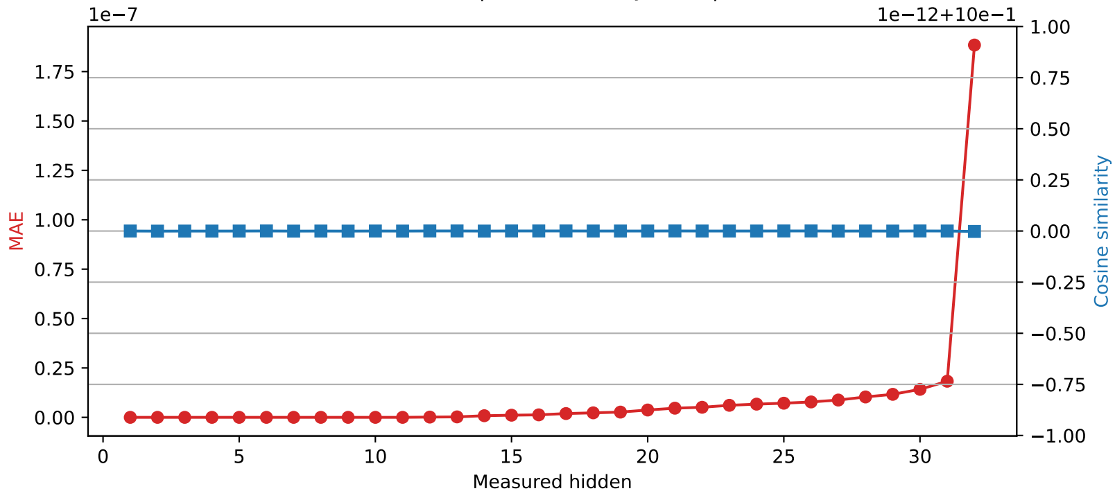
Mistral-7B-Instruct-v0.3 | Quantized layer 11 | float64 → int32
