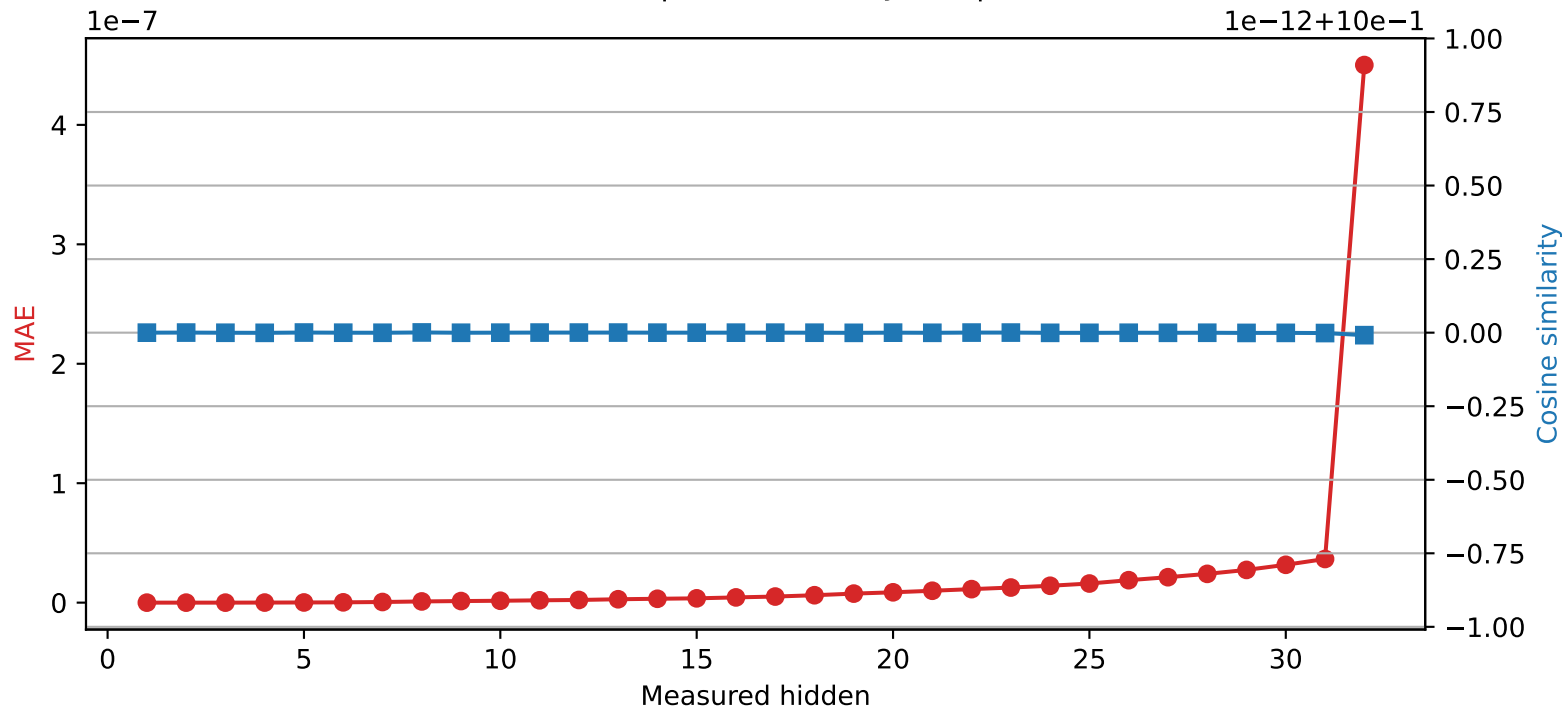
Mistral-7B-Instruct-v0.3 | Quantized layer 3 | float64 → int32
