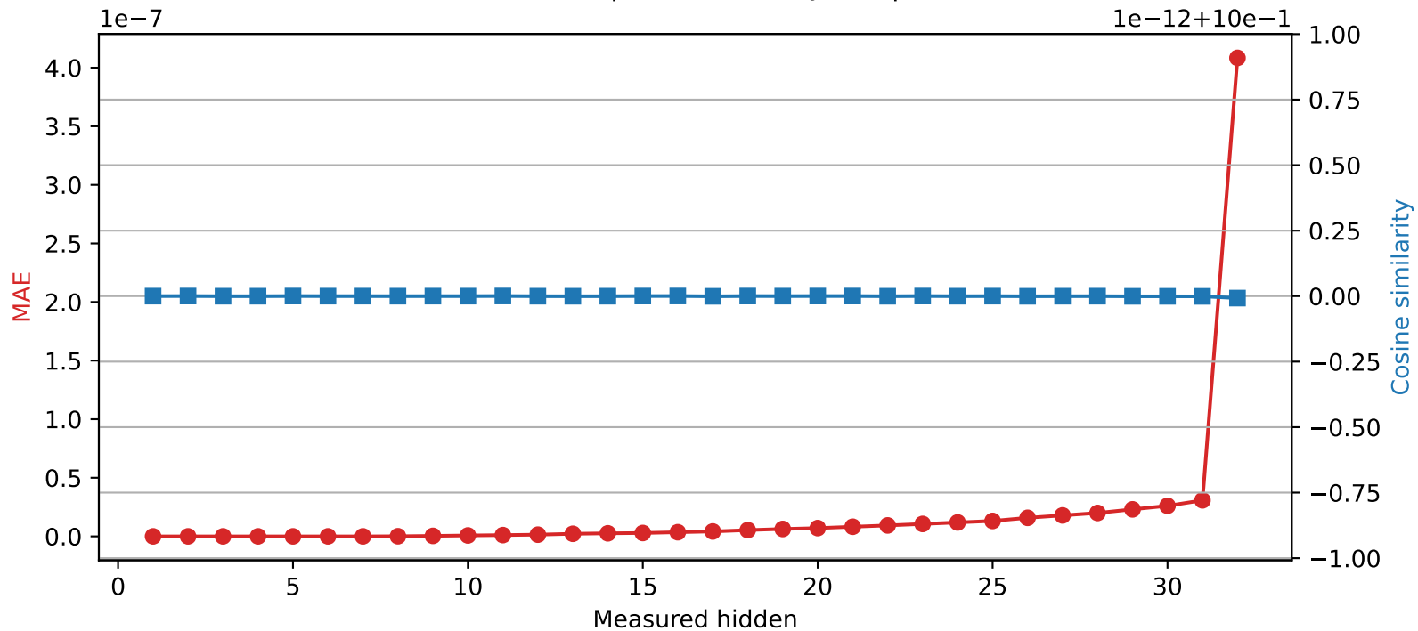
Mistral-7B-Instruct-v0.3 | Quantized layer 7 | float64 → int32
