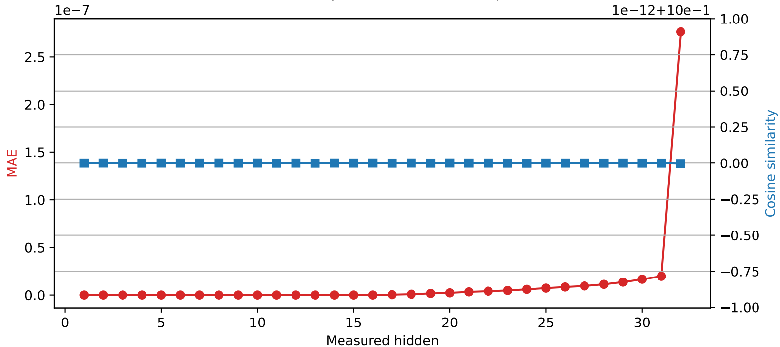
Mistral-7B-Instruct-v0.3 | Quantized layer 16 | float64 → int32
