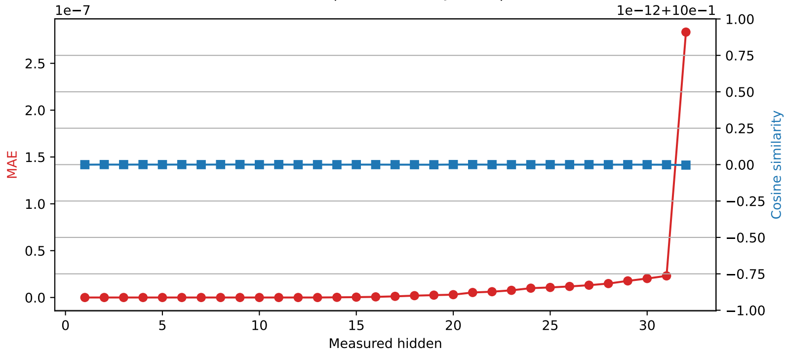
Mistral-7B-Instruct-v0.3 | Quantized layer 13 | float64 → int32
