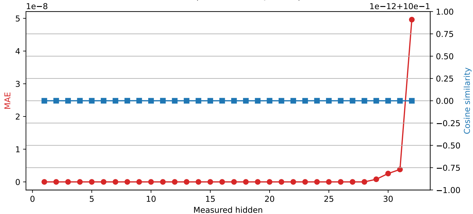
Mistral-7B-Instruct-v0.3 | Quantized layer 28 | float64 → int32
