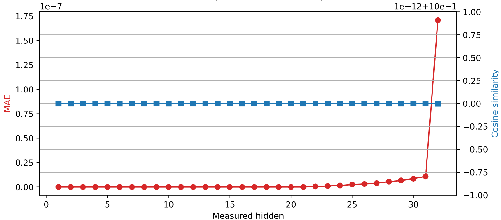
Mistral-7B-Instruct-v0.3 | Quantized layer 21 | float64 → int32
