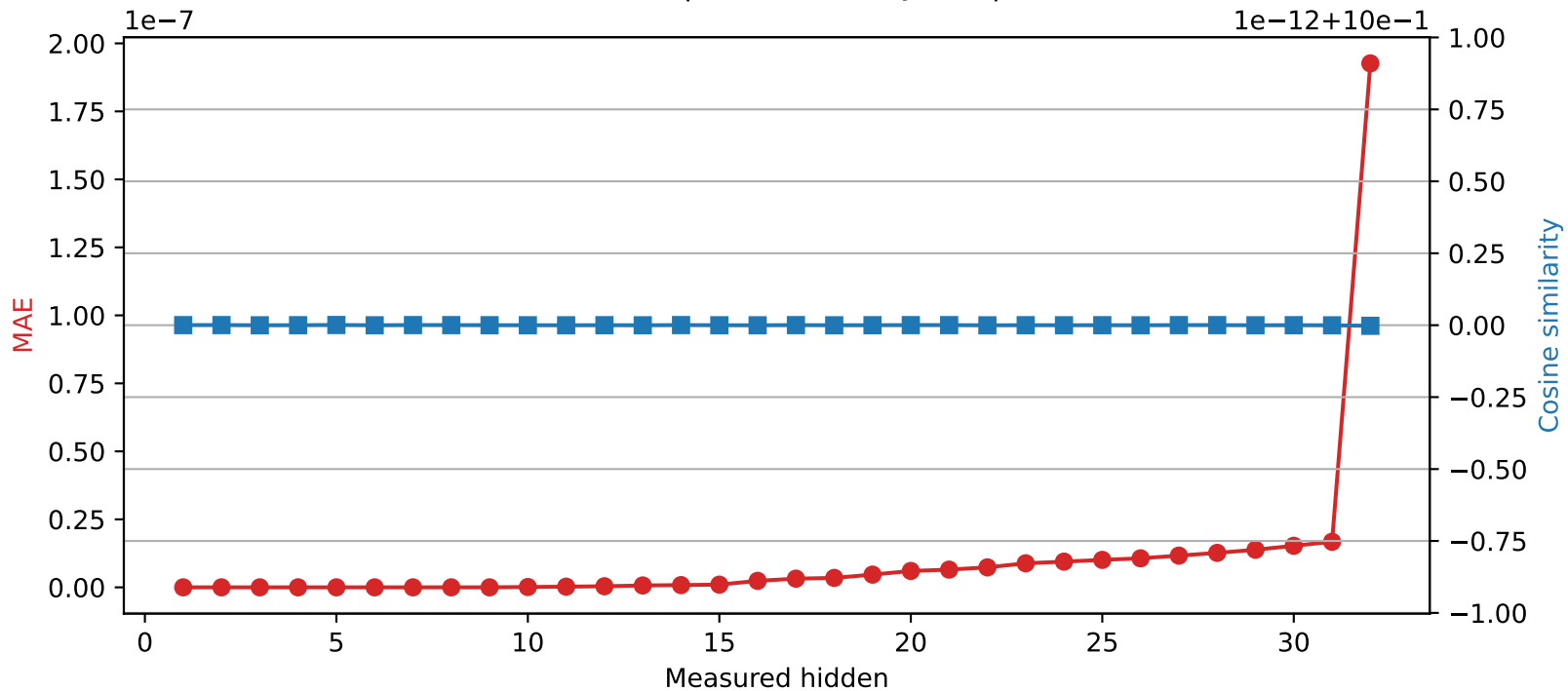
Mistral-7B-Instruct-v0.3 | Quantized layer 9 | float64 \rightarrow int32
