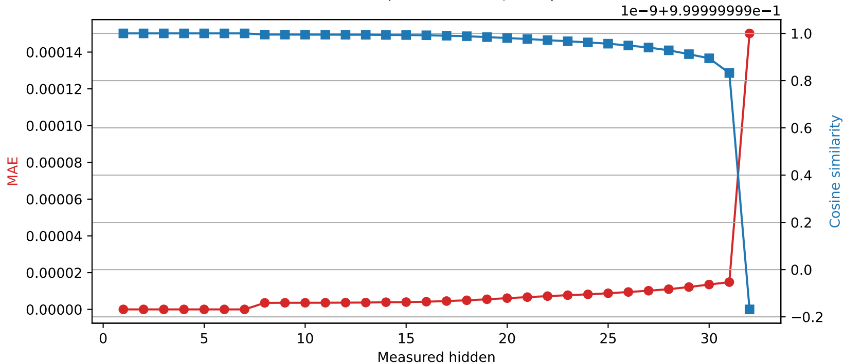
Mistral-7B-Instruct-v0.3 | Quantized layer 7 | float32 \rightarrow int16
