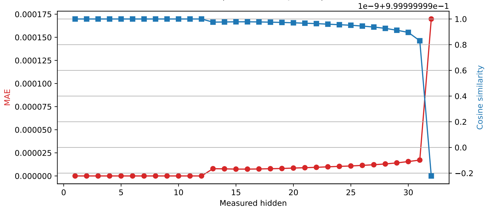
Mistral-7B-Instruct-v0.3 | Quantized layer 12 | float32 → int16
