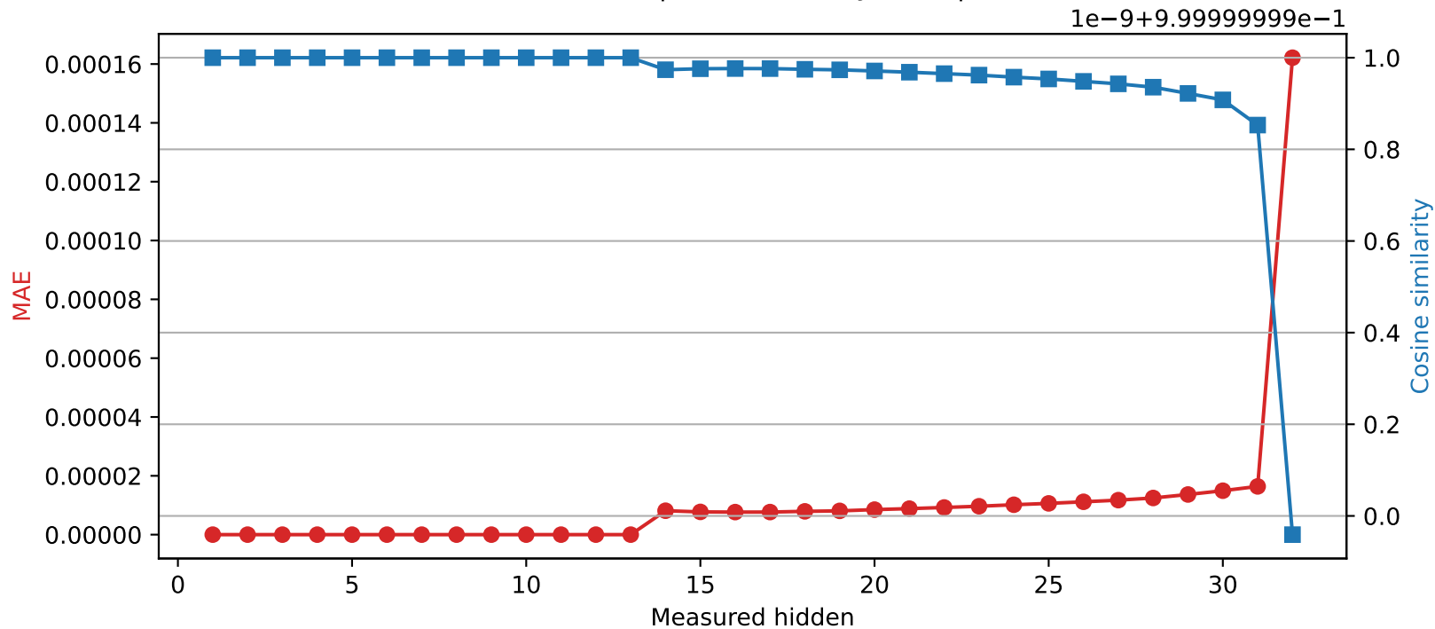
Mistral-7B-Instruct-v0.3 | Quantized layer 13 | float32 → int16
