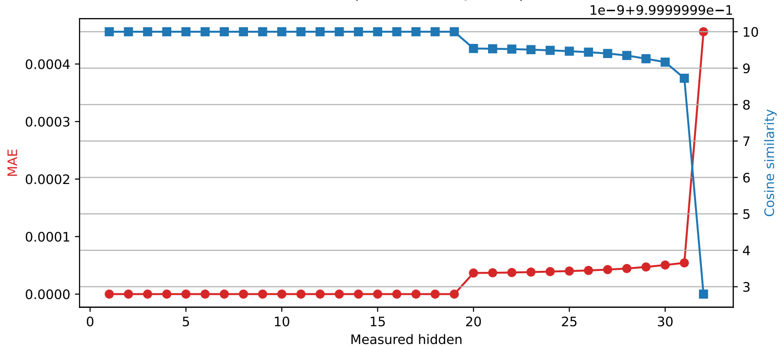
Mistral-7B-Instruct-v0.3 | Quantized layer 19 | float32 → int16
