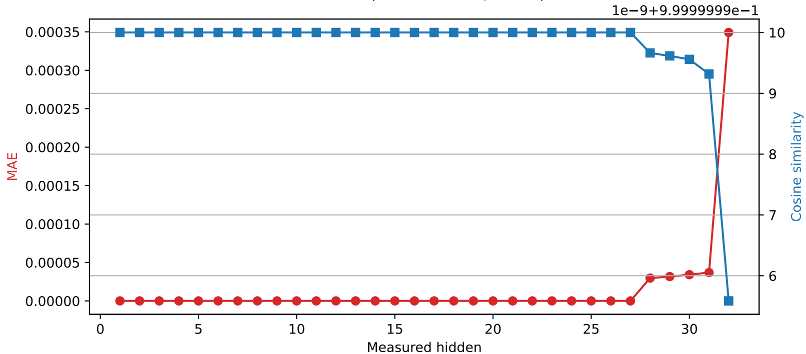
Mistral-7B-Instruct-v0.3 | Quantized layer 27 | float32 → int16
