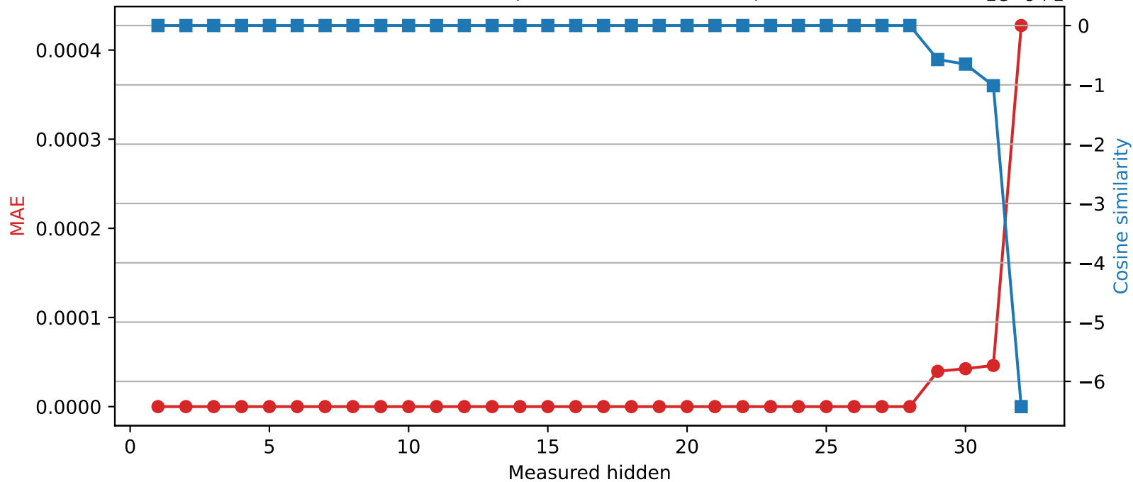
Mistral-7B-Instruct-v0.3 | Quantized layer 28 | float32 \rightarrow int16
