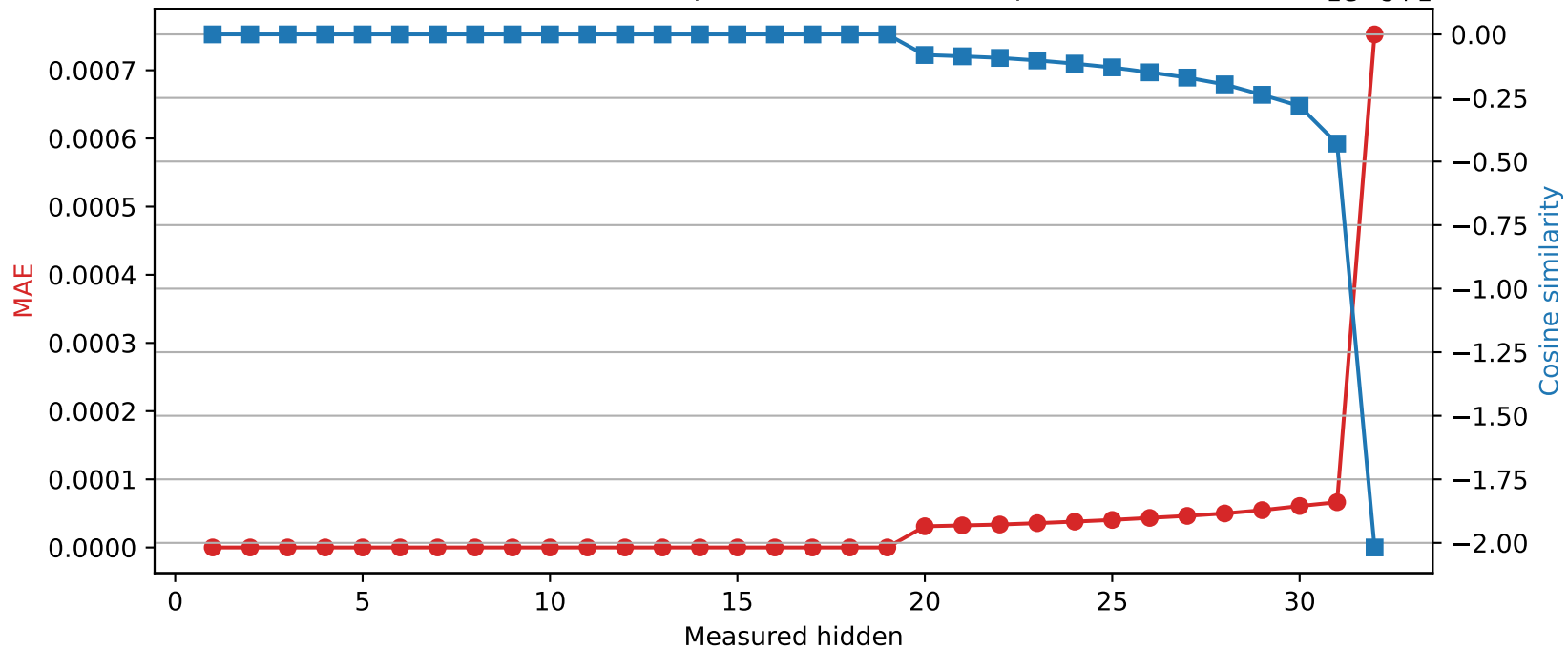
Mistral-7B-Instruct-v0.3 | Quantized layer 19 | float32 \rightarrow int16
