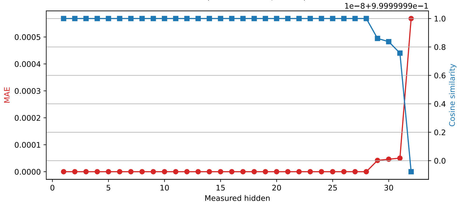
Mistral-7B-Instruct-v0.3 | Quantized layer 28 | float32 → int16
