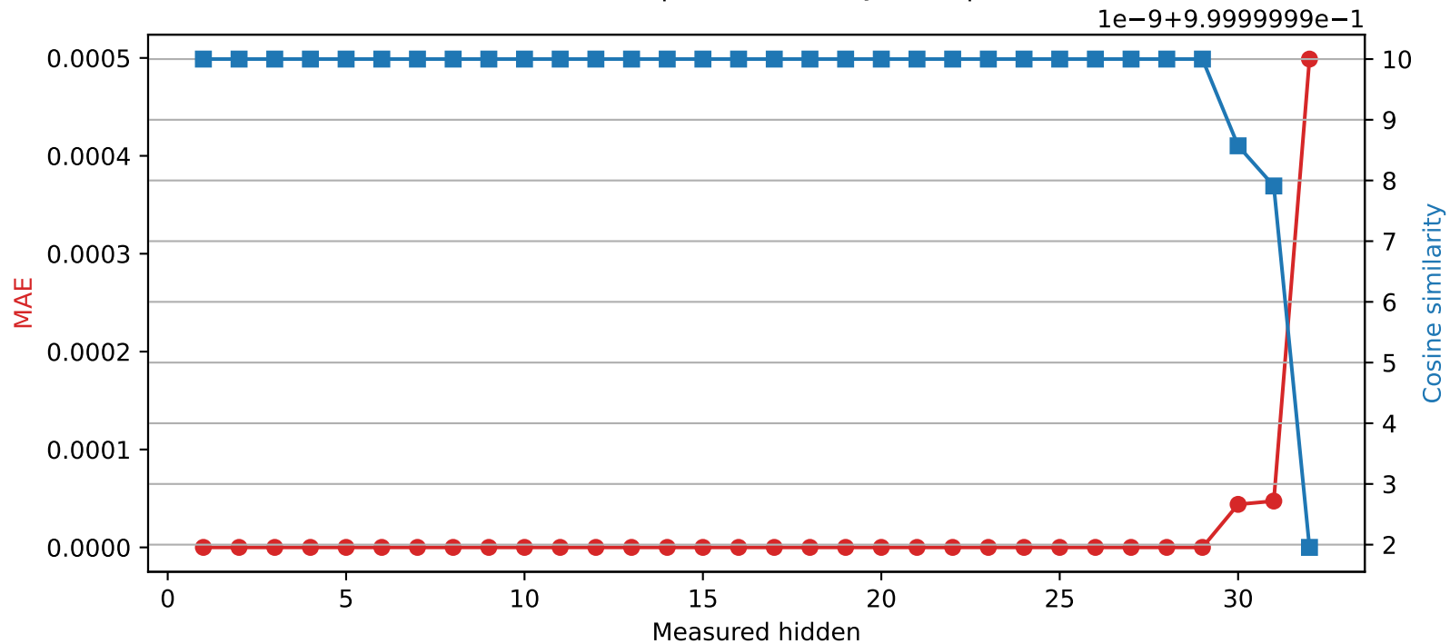
Mistral-7B-Instruct-v0.3 | Quantized layer 29 | float32 → int16
