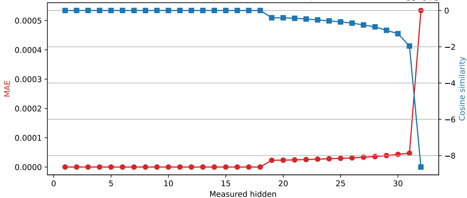
Mistral-7B-Instruct-v0.3 | Quantized layer 18 | float32 → int16
