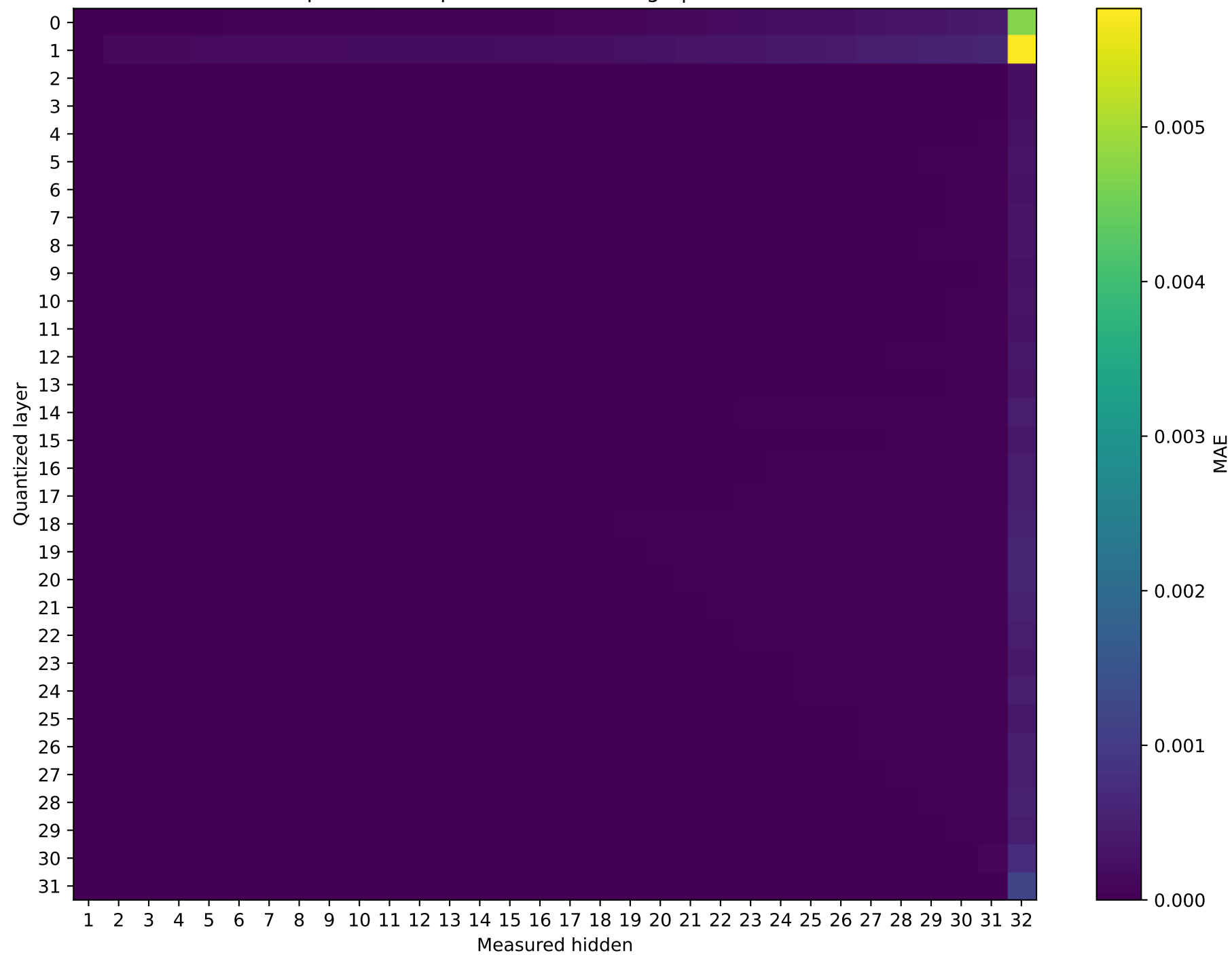
Mistral-7B-Instruct-v0.3 Prompt 3: MAE representation damage | float32 → int16
