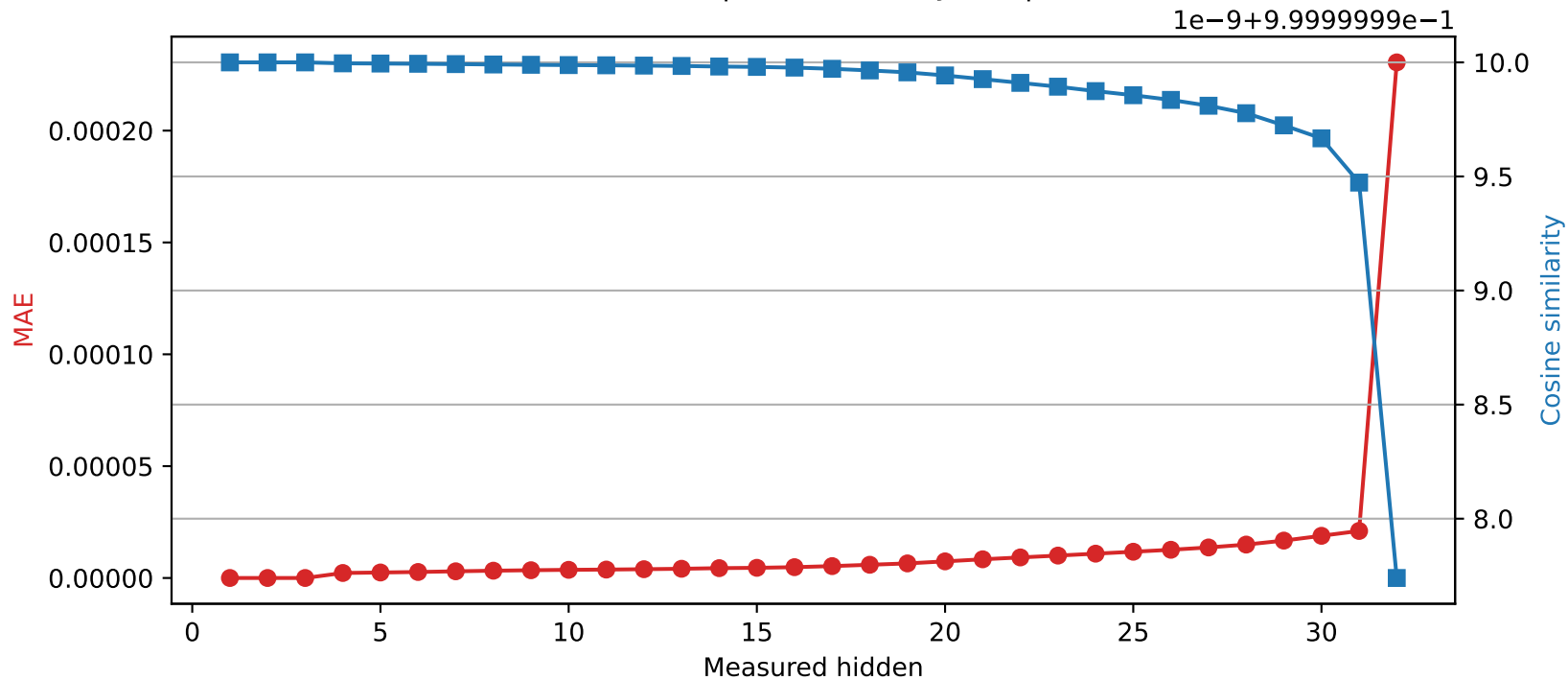
Mistral-7B-Instruct-v0.3 | Quantized layer 3 | float32 \rightarrow int16
