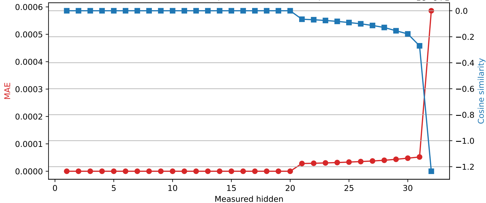
Mistral-7B-Instruct-v0.3 | Quantized layer 20 | float32 \rightarrow int16
