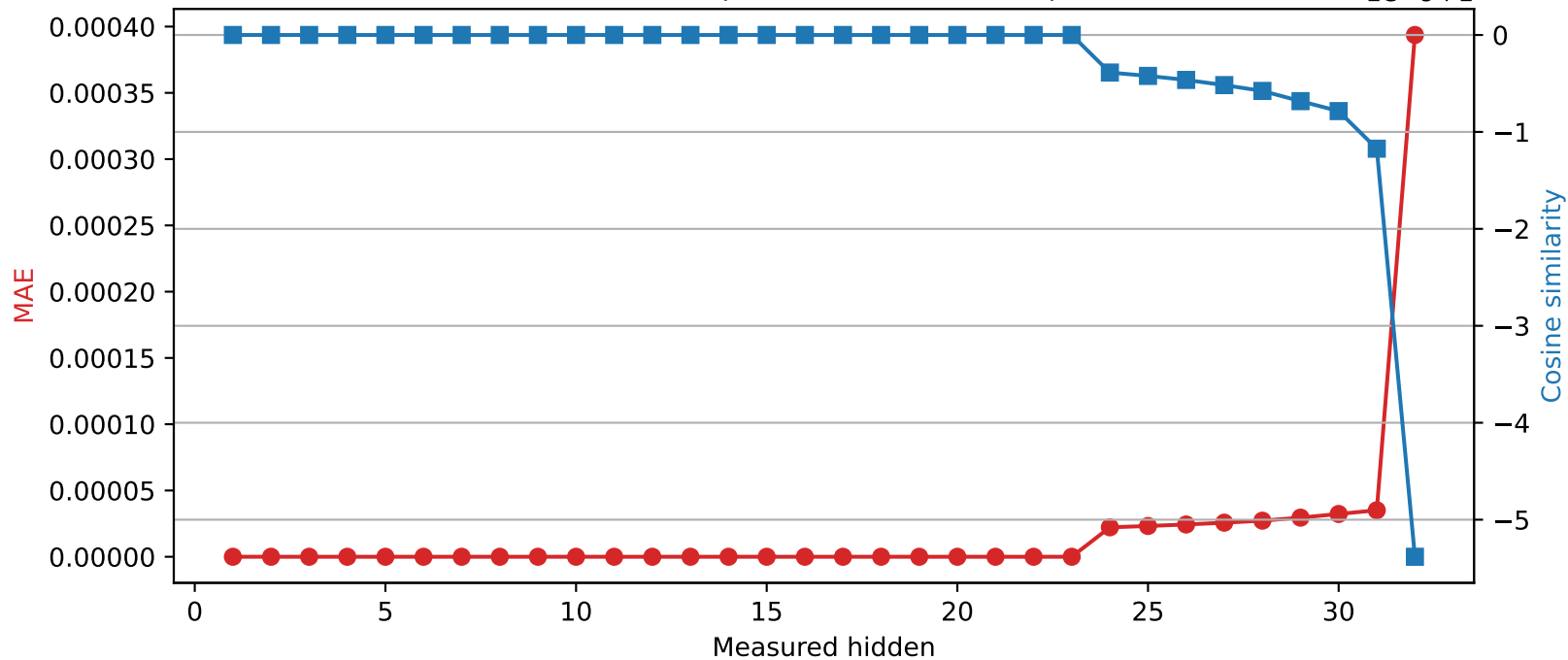
Mistral-7B-Instruct-v0.3 | Quantized layer 23 | float32 → int16
