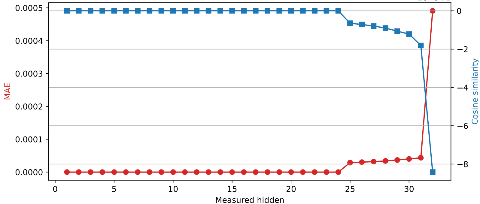
Mistral-7B-Instruct-v0.3 | Quantized layer 24 | float32 \rightarrow int16
