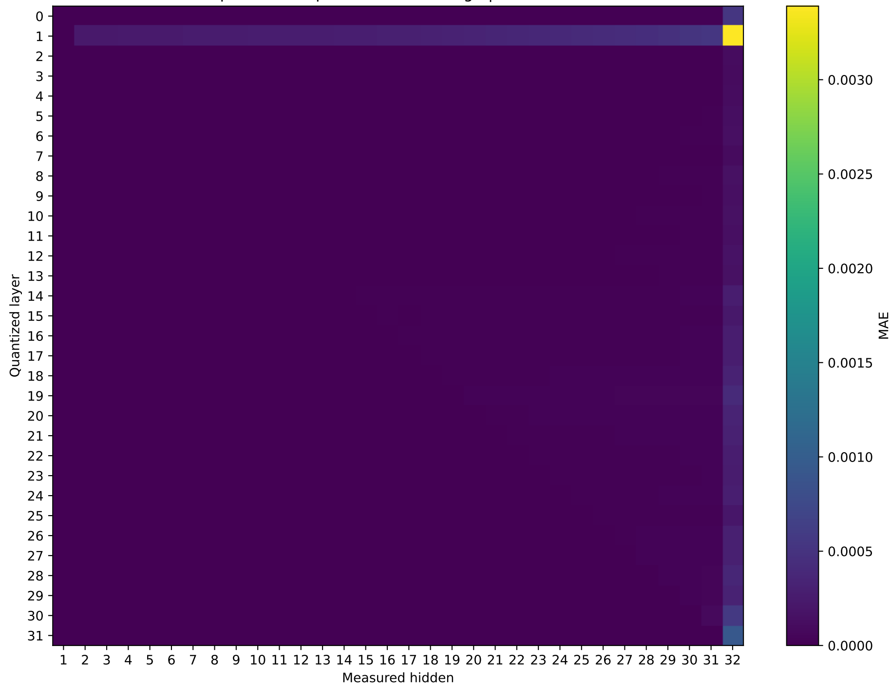
Mistral-7B-Instruct-v0.3 Prompt 4: MAE representation damage | float32 → int16
