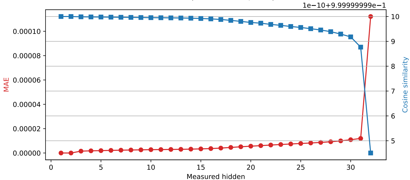
Mistral-7B-Instruct-v0.3 | Quantized layer 2 | float32 \rightarrow int16
