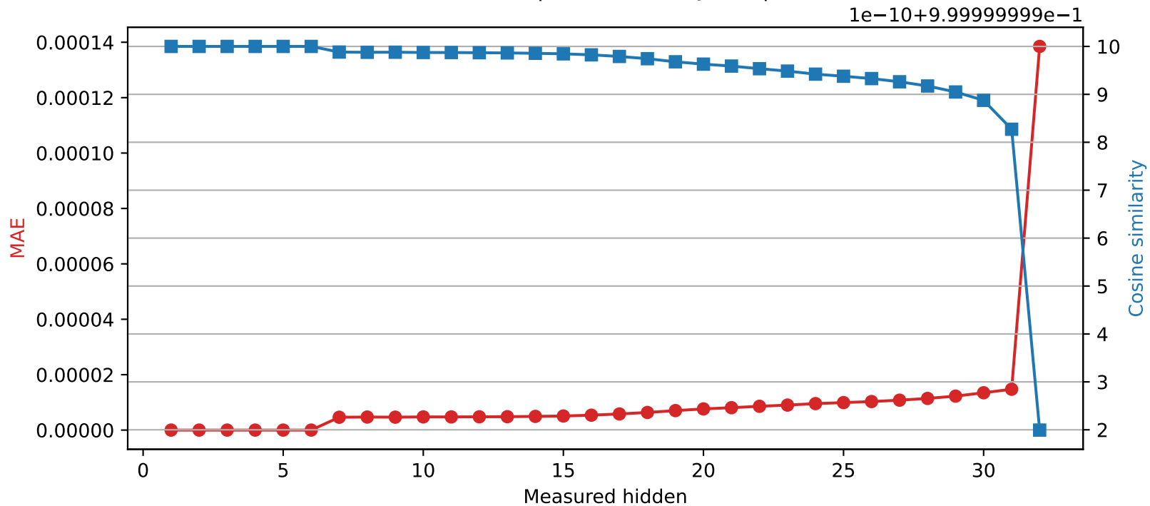
Mistral-7B-Instruct-v0.3 | Quantized layer 6 | float32 → int16
