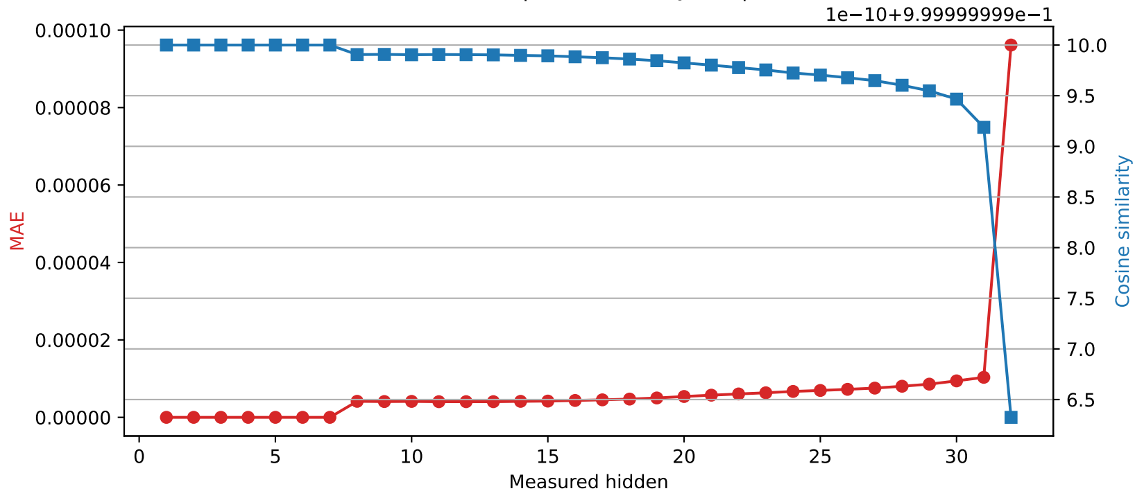
Mistral-7B-Instruct-v0.3 | Quantized layer 7 | float32 → int16
