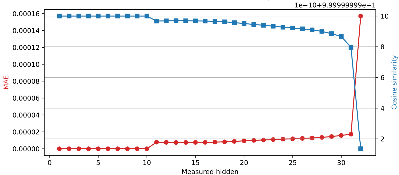
Mistral-7B-Instruct-v0.3 | Quantized layer 10 | float32 → int16
