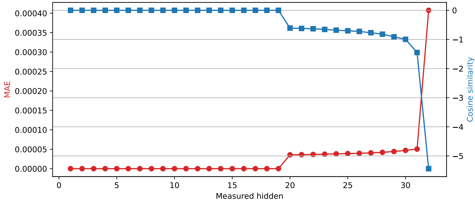
Mistral-7B-Instruct-v0.3 | Quantized layer 19 | float32 → int16
