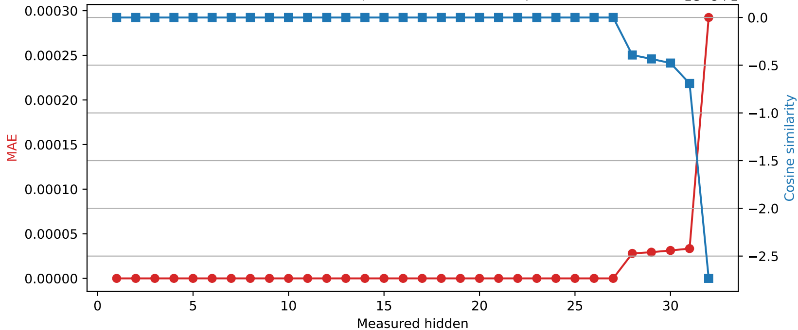
Mistral-7B-Instruct-v0.3 | Quantized layer 27 | float32 → int16
