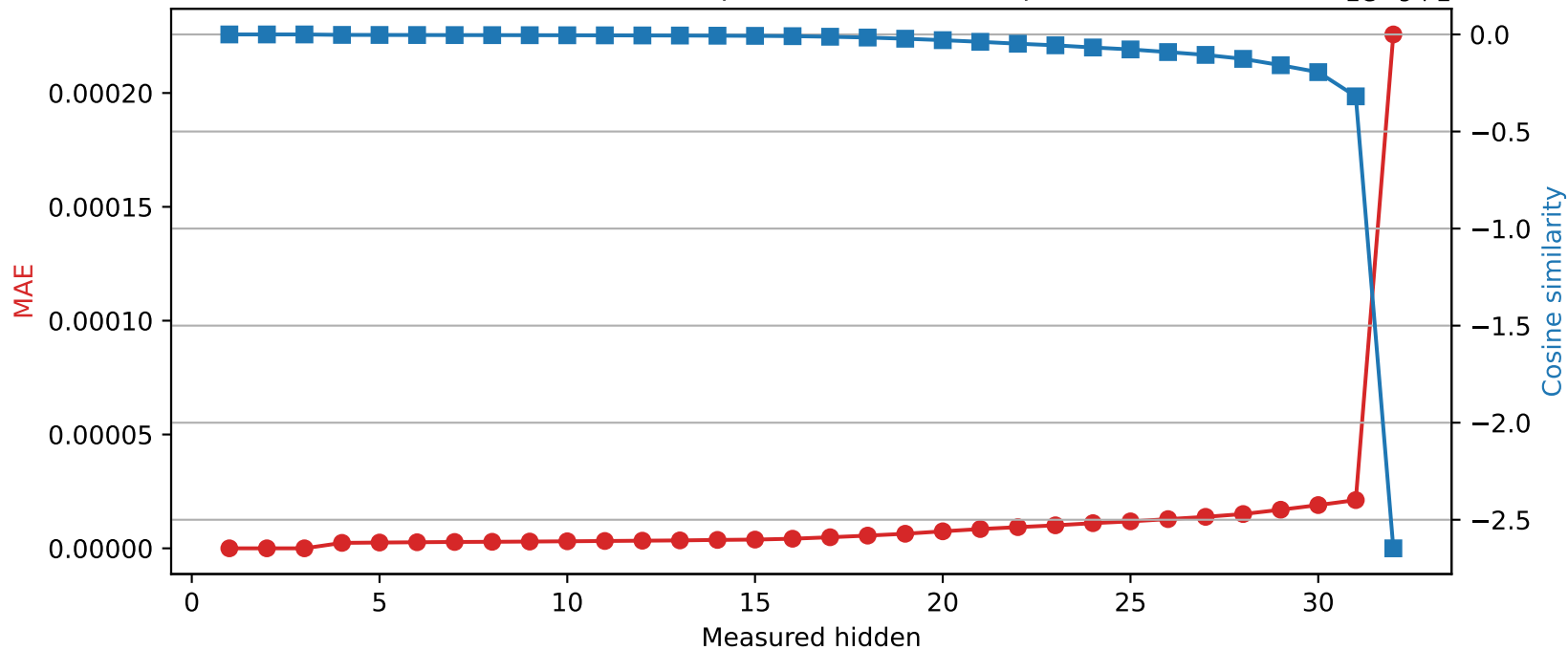
Mistral-7B-Instruct-v0.3 | Quantized layer 3 | float64 → int16
