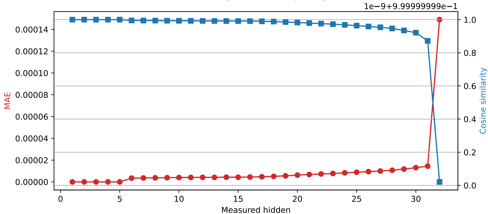
Mistral-7B-Instruct-v0.3 | Quantized layer 5 | float64 → int16
