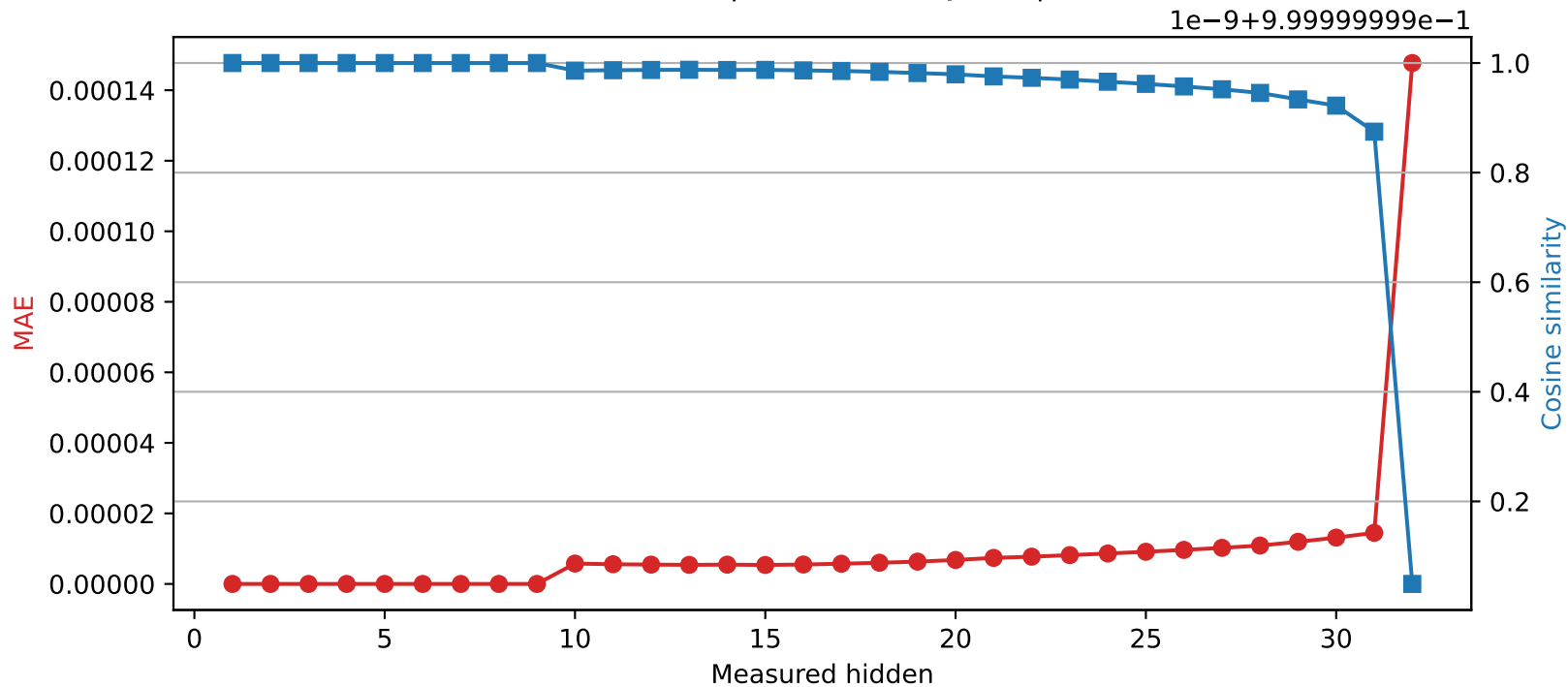
Mistral-7B-Instruct-v0.3 | Quantized layer 9 | float64 → int16
