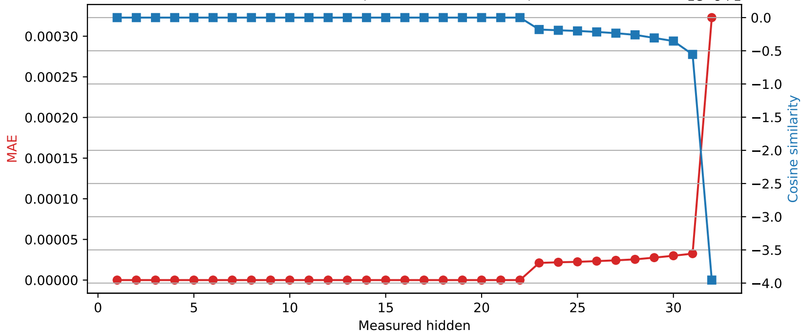
Mistral-7B-Instruct-v0.3 | Quantized layer 22 | float64 → int16
