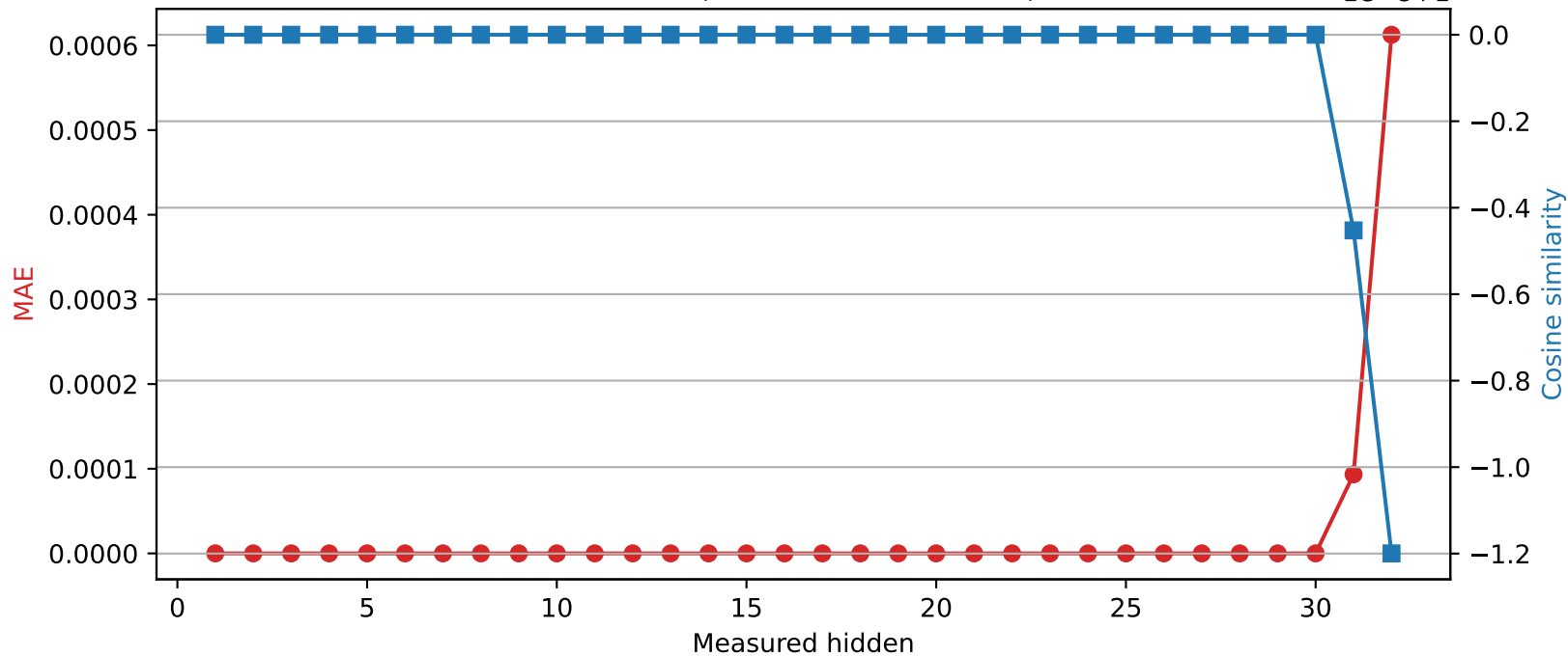
Mistral-7B-Instruct-v0.3 | Quantized layer 30 | float64 → int16
