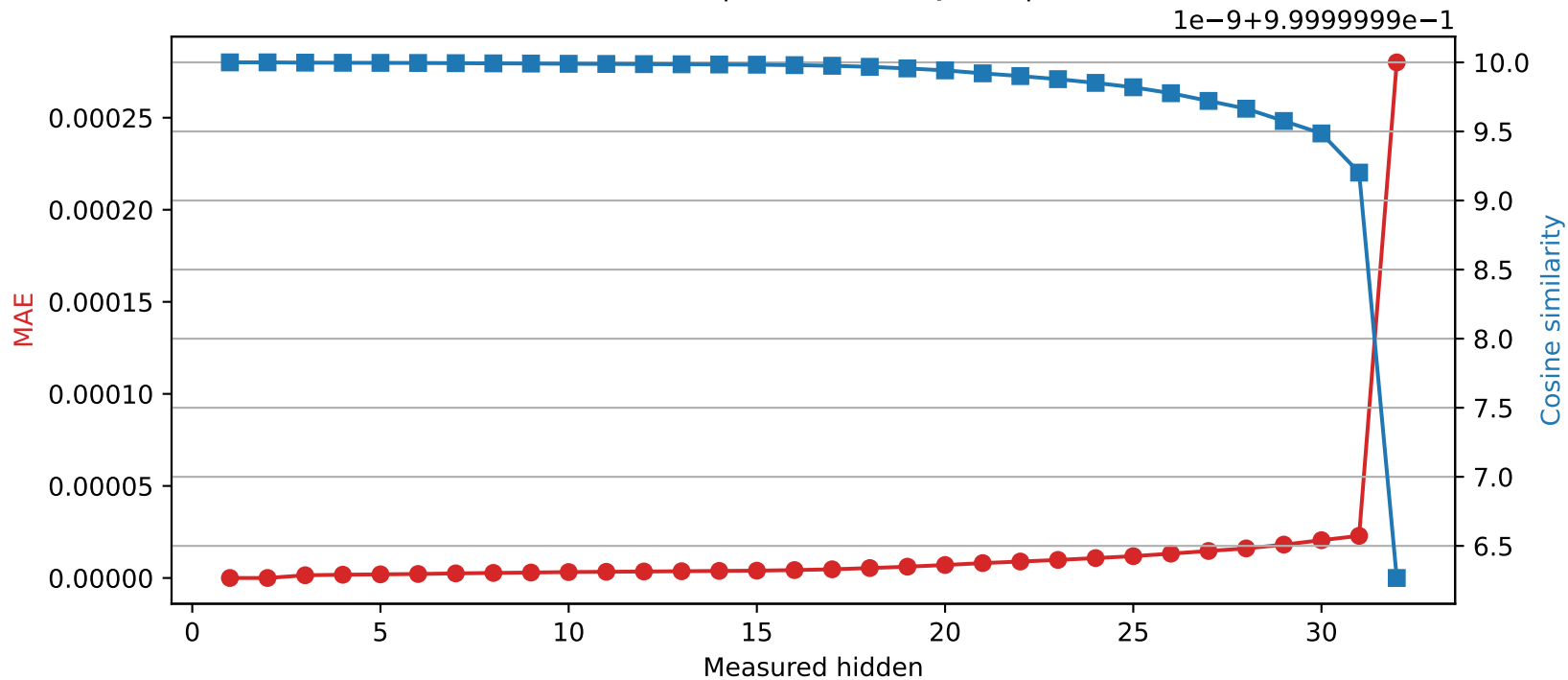
Mistral-7B-Instruct-v0.3 | Quantized layer 2 | float64 → int16
