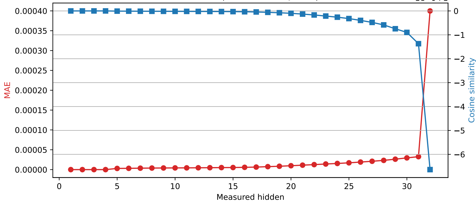
Mistral-7B-Instruct-v0.3 | Quantized layer 4 | float64 → int16
