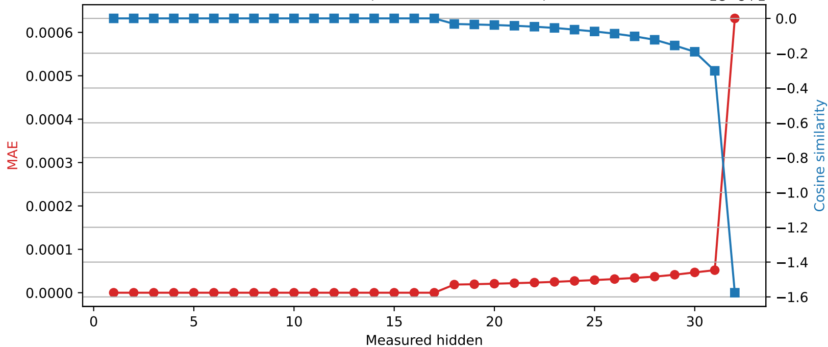
Mistral-7B-Instruct-v0.3 | Quantized layer 17 | float64 → int16
