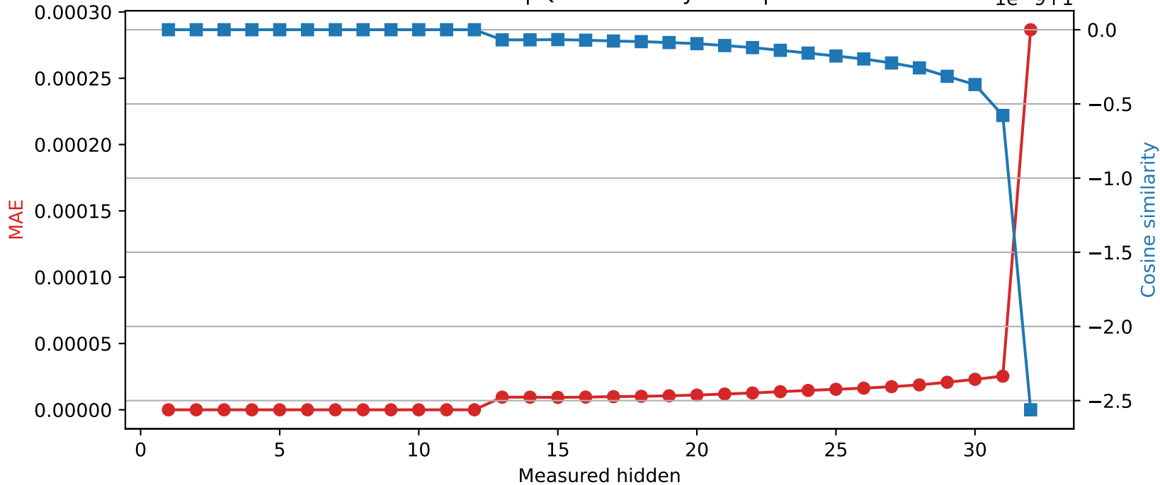
Mistral-7B-Instruct-v0.3 | Quantized layer 12 | float64 → int16
