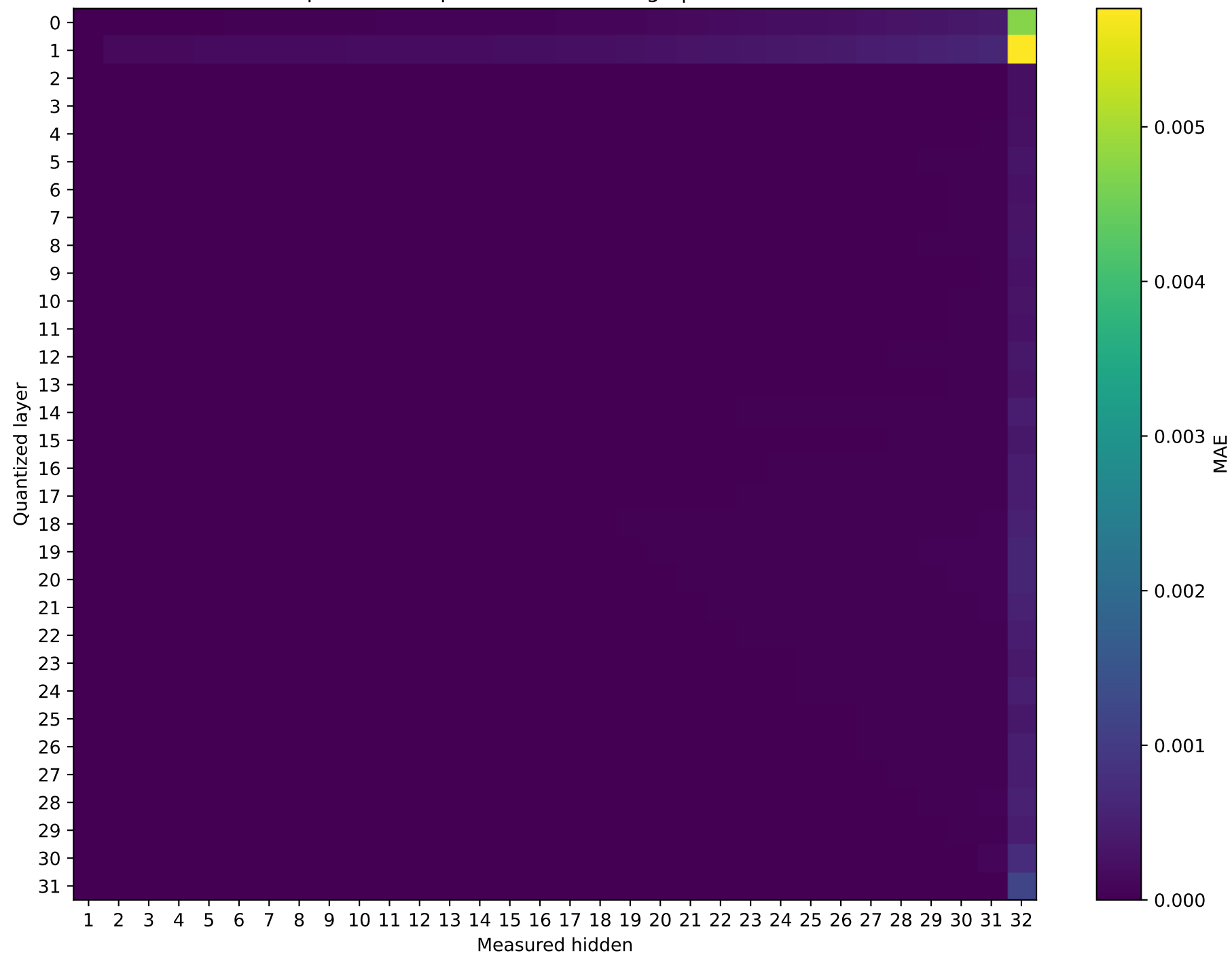
Mistral-7B-Instruct-v0.3 Prompt 3: MAE representation damage | float64 → int16
