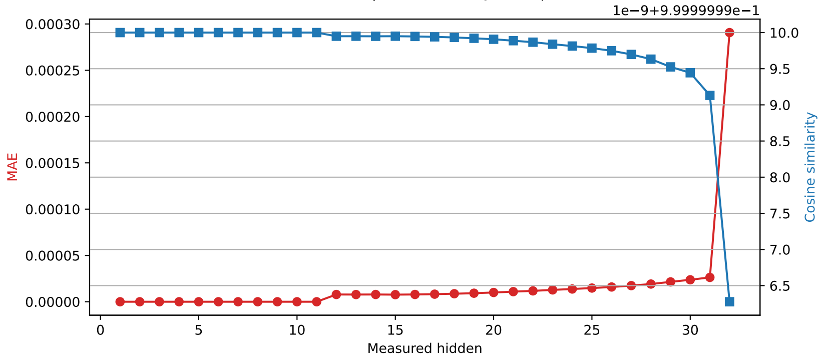
Mistral-7B-Instruct-v0.3 | Quantized layer 11 | float64 → int16
