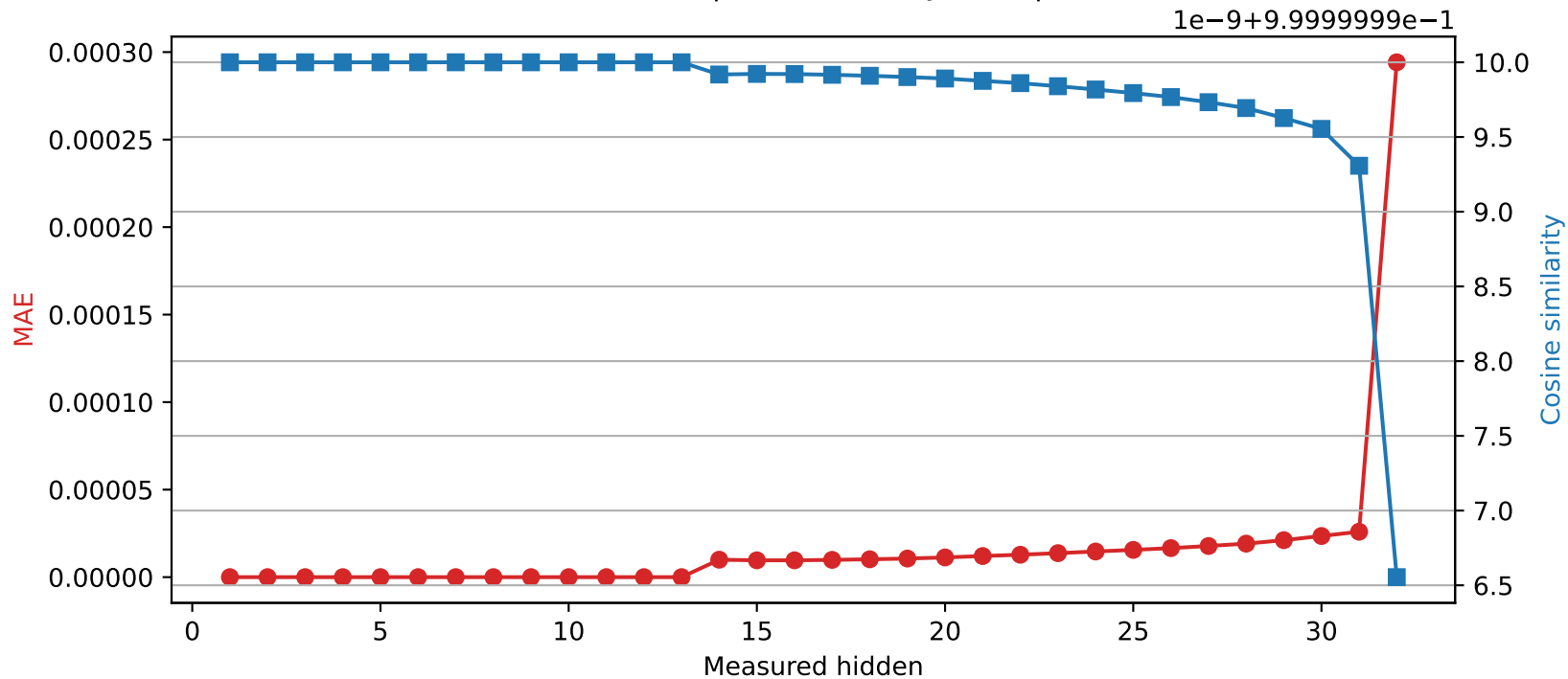
Mistral-7B-Instruct-v0.3 | Quantized layer 13 | float64 → int16
