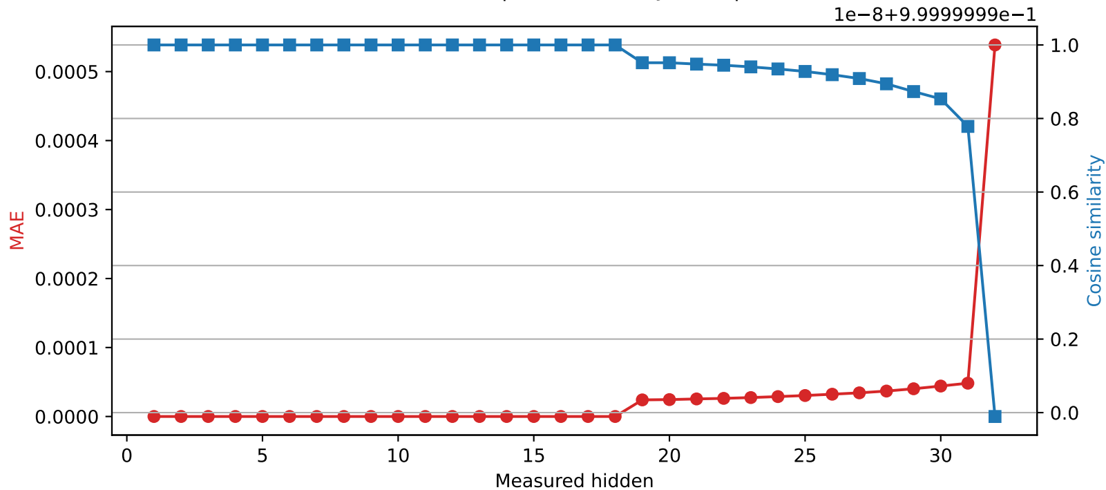
Mistral-7B-Instruct-v0.3 | Quantized layer 18 | float64 → int16
