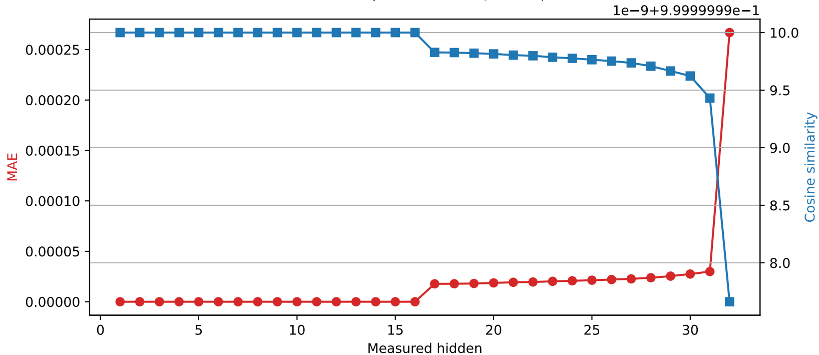
Mistral-7B-Instruct-v0.3 | Quantized layer 16 | float64 → int16
